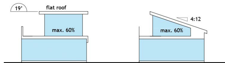
Figure 3: Building height and partial second storey for roofs less than 7:12
