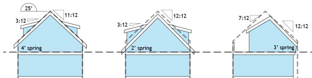
Figure 2: Building height and partial second storey for pitched roofs 7:12 or greater
