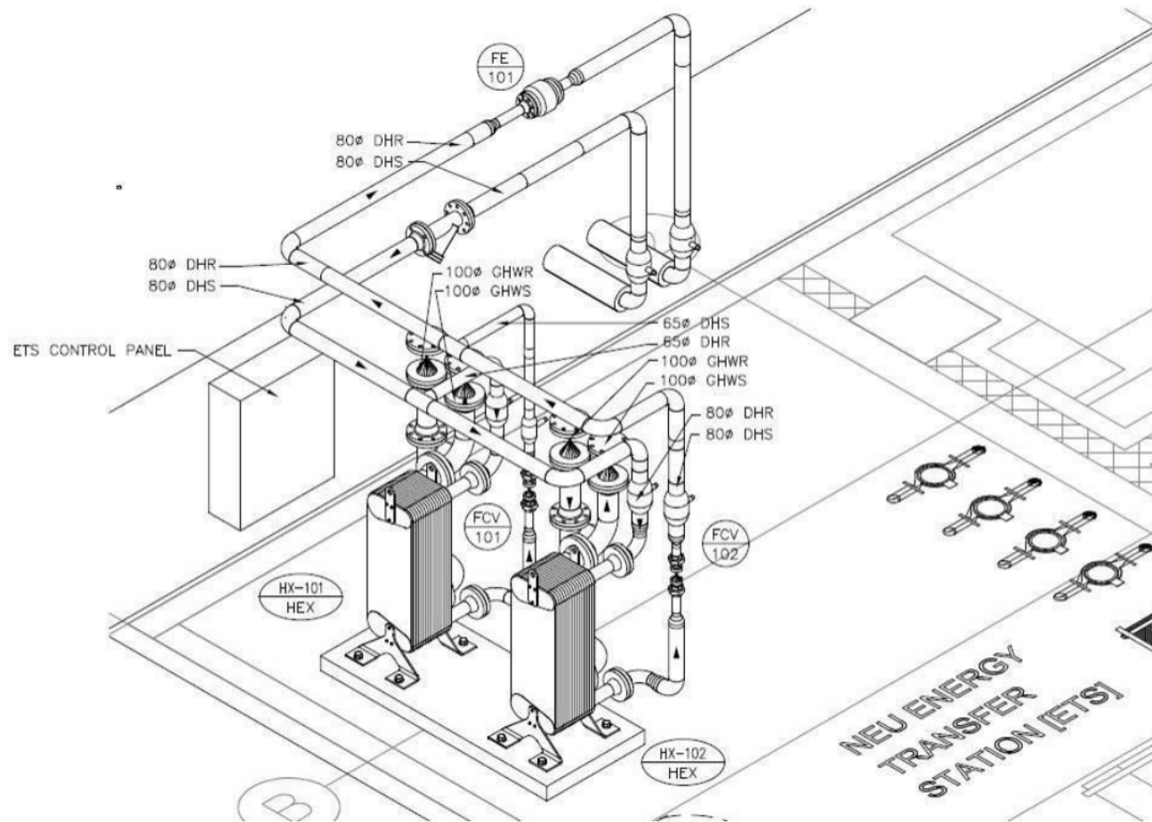
Figure 2: Typical ETS Configuration
