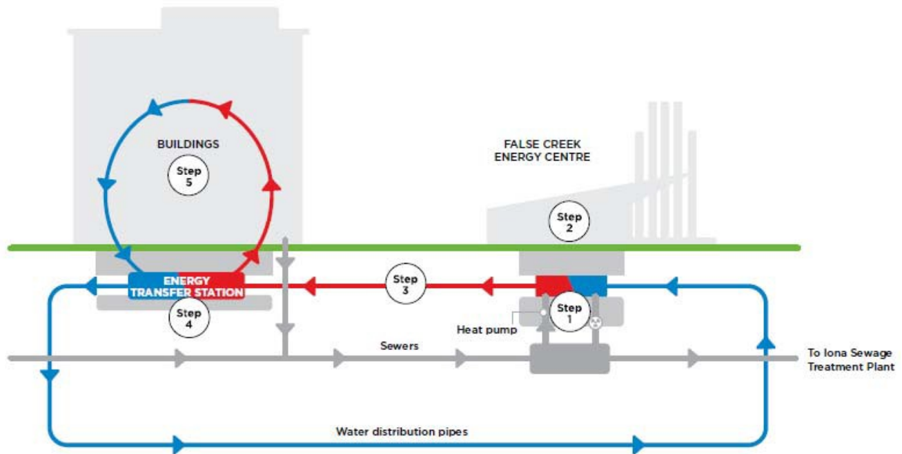
Figure 1: The NEU System Components
