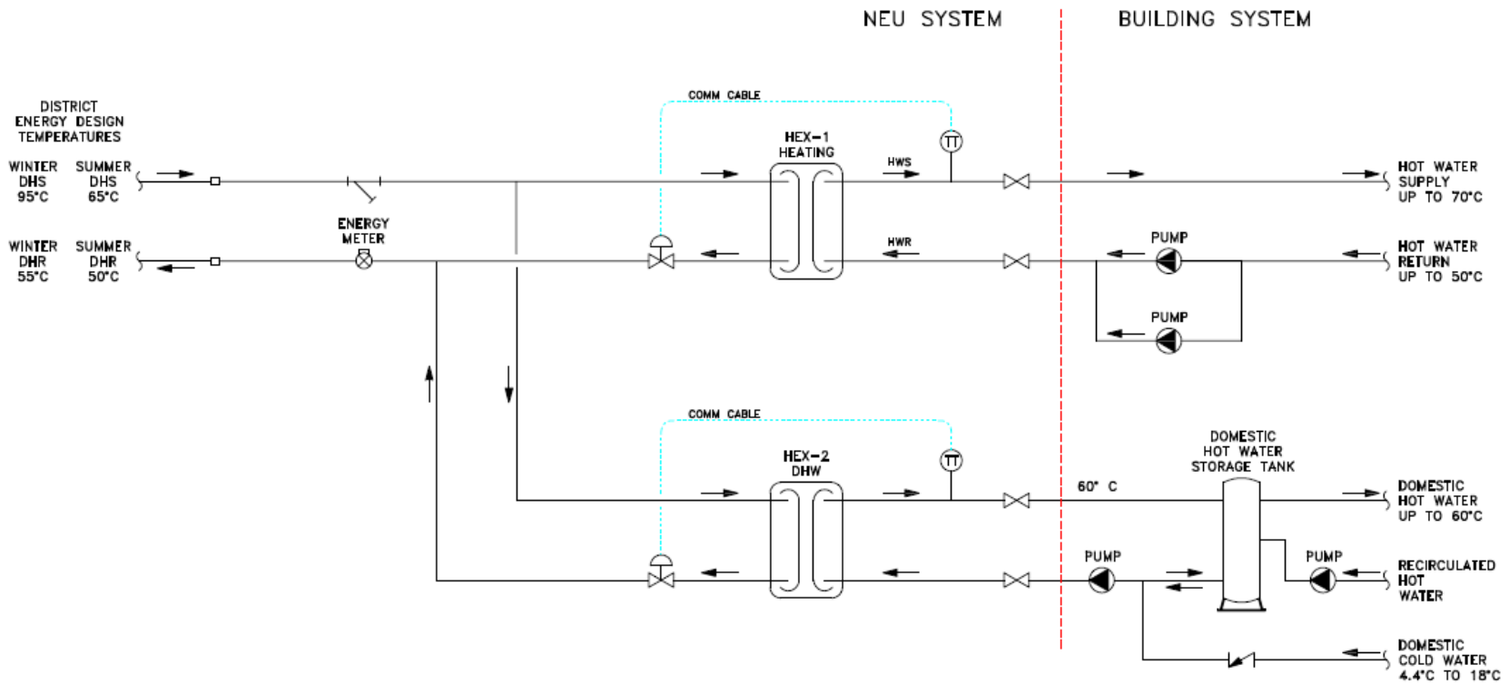
Figure 3: Typical ETS Schematic and Building Connection
