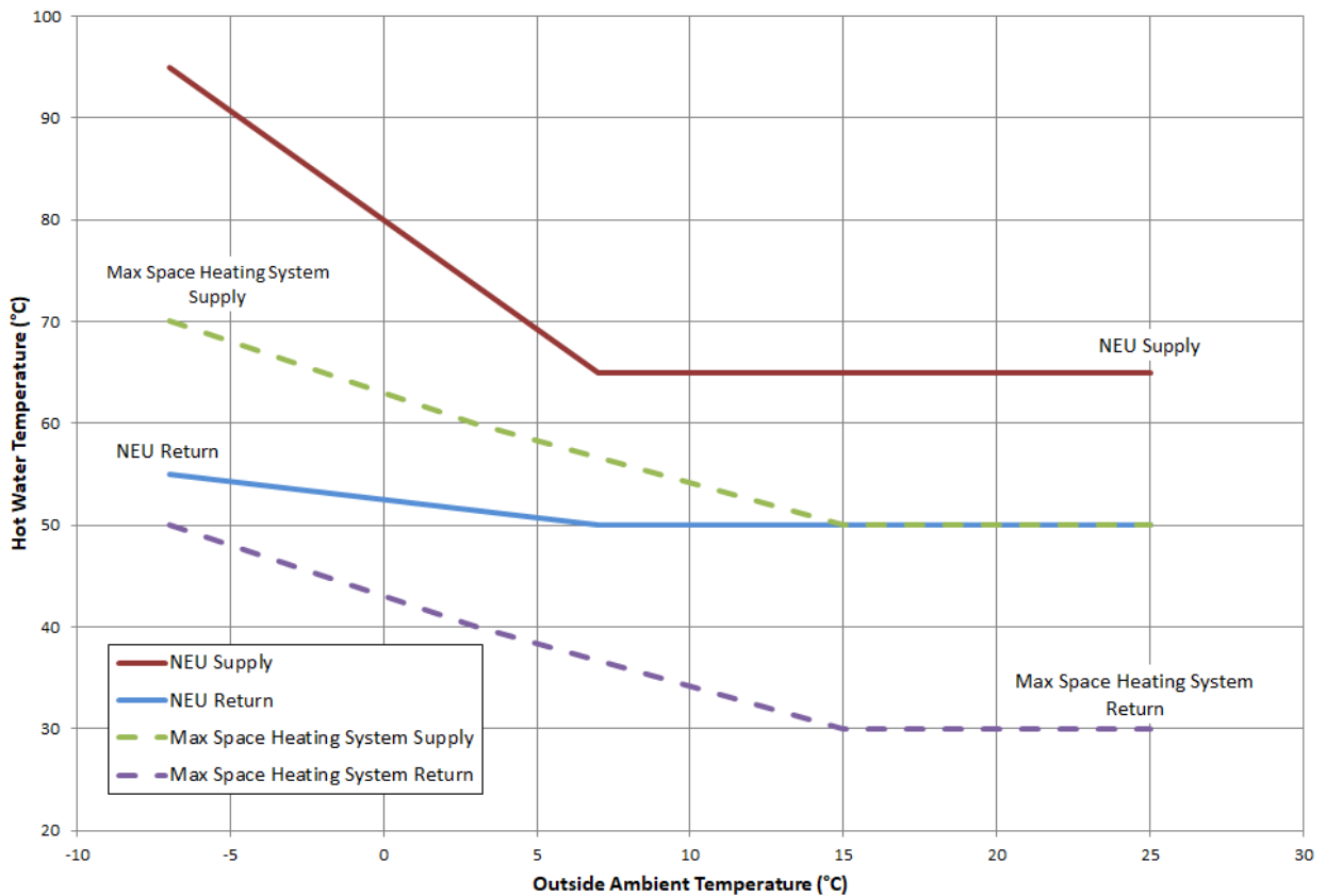
Figure 4: NEU System and Building Heating System Temperatures
