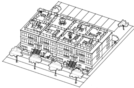
Figure 1: Illustration of back-to-back arrangement of stacked townhouses or rowhouses
