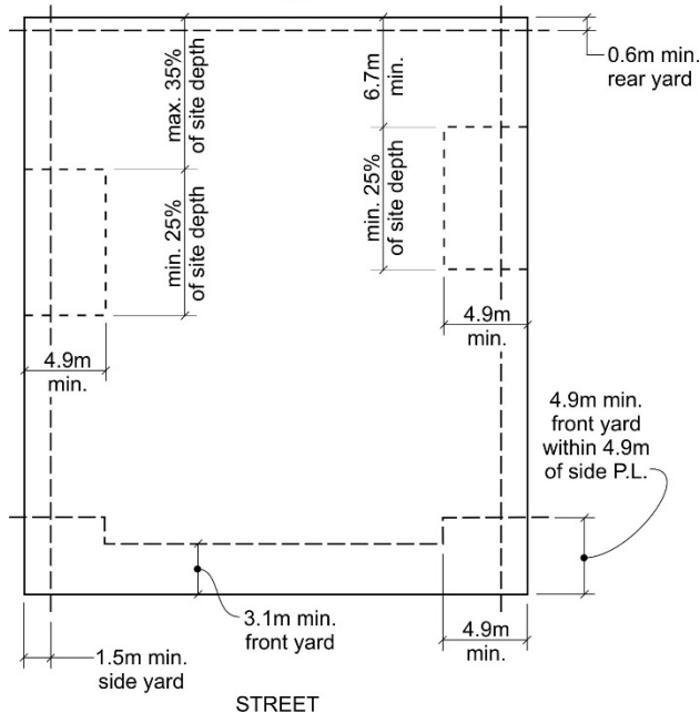
Figure 14: Minimum yards diagram for townhouse in a courtyard configuration
