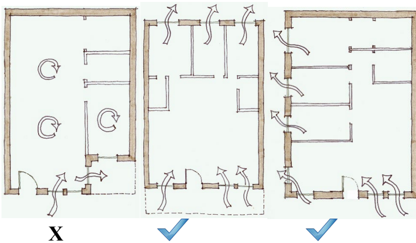
Figure 8: Dwelling Unit with a single exposure lacks the opportunity for natural displacement of indoor air (left) vs dwelling units with two exposures (right)
