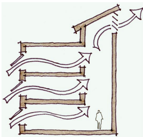
Figure 9: Stack effect
